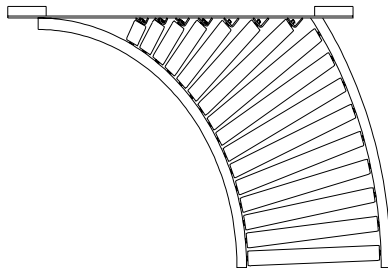
Curved Spur 90° (3" Roller Centers Only)
