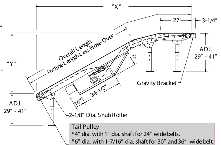
8" Center Drive Double Nose-Over - (Guarding removed for clarity.)
